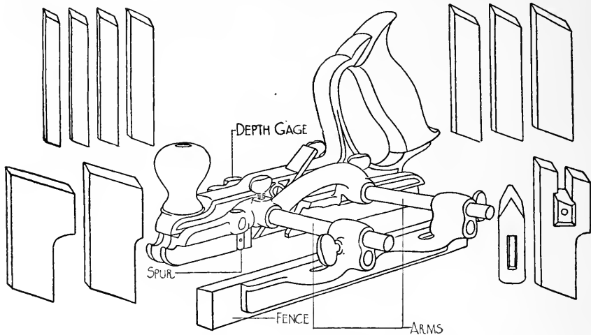
FIG. 72. PLOW AND MATCHING PLANE.
